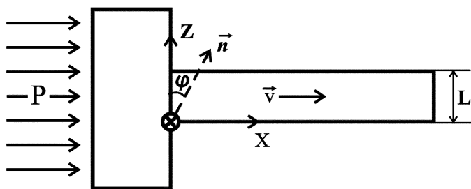
FIGURE 1 Considered cell: P is the radiation intensity, \vec{v} is the flow velocity, L is the thickness of capillary and \vec{n} is the NLC director.
