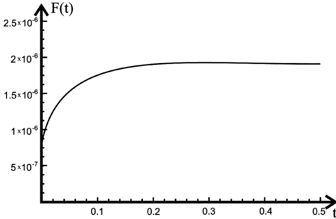
FIGURE 8 Deformation free energy of the hybrid oriented liquid crystal cells after switching the laser radiation “on”.
