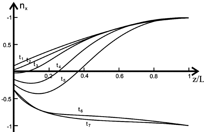
FIGURE 9 Profile of the director’s x component ( n_x ) for different times ( t_j ) after switching the laser radiation “on” for hybrid oriented cells in the case of the generalized problem ( t_1 = 0 sec, t_2 = 3.8 \cdot 10^{-5} sec, t_3 = 1.14 \cdot 10^{-4} sec, t_4 = 1.9 \cdot 10^{-4} sec, t_5 = 3.8 \cdot 10^{-4} sec, t_6 = 1.14 \cdot 10^{-3} sec, t_7 = 3.8 \cdot 10^{-3} sec). Reversal time is: t_\tau \approx 0.67 \cdot 10^{-3} sec.
