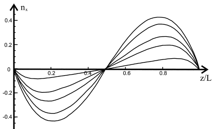
FIGURE 5 Profile of the director's x component ( n_x ) for different times ( t_j ) after switching the laser radiation "on" for homeotropic oriented cell with an approximation of strong anchoring. ( t_1 = 0 sec, t_2 = 2.28 \cdot 10^{-5} sec, t_3 = 0.68 \cdot 10^{-4} sec, t_4 = 1.14 \cdot 10^{-4} sec, t_5 = 2.28 \cdot 10^{-4} sec, t_6 = 2.28 \cdot 10^{-3} sec).
