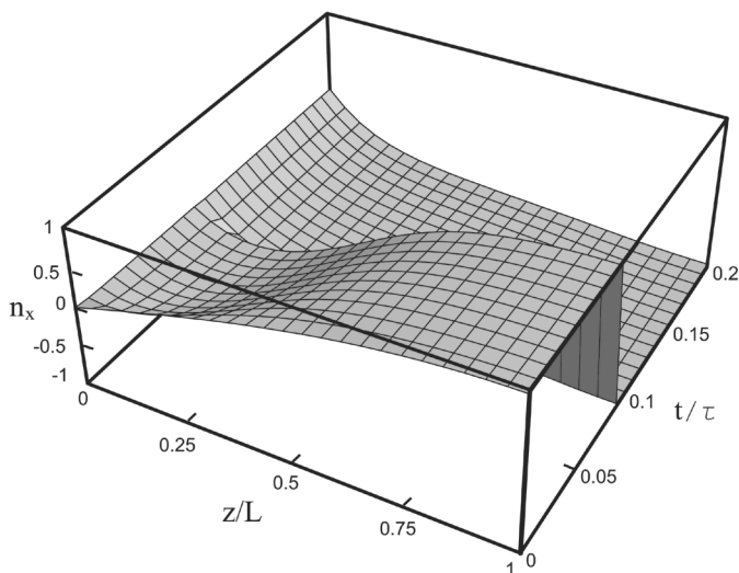
FIGURE 10 Three-dimensional time and space dependence of the director's x component after switching the laser radiation "on"; for hybrid oriented cells in the case of the generalized problem.
