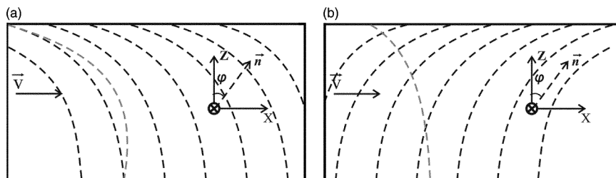
FIGURE 3 Director profile in hybrid oriented cells with nematic LC.
