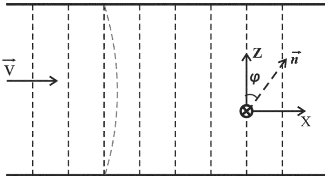
FIGURE 2 Director profile in a homeotropic oriented cell with nematic LC.
