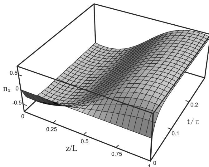
FIGURE 6 Three-dimensional time and space dependence of the director's x component after switching the laser radiation "on"; for homeotropic oriented cells in the case of the generalized problem.
