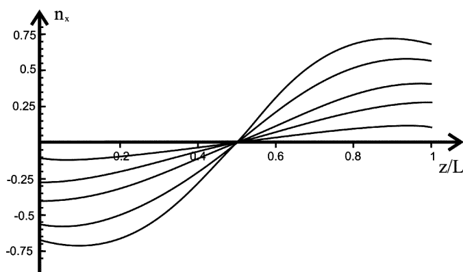
FIGURE 7 Profile of the director's x component ( n_x ) for different times ( t_j ) after switching the laser radiation "on" for homeotropic oriented cells in the case of the generalized problem. ( t_1 = 0 sec, t_2 = 2.28 \cdot 10^{-5} sec, t_3 = 0.68 \cdot 10^{-4} sec, t_4 = 1.14 \cdot 10^{-4} sec, t_5 = 2.28 \cdot 10^{-4} sec, t_6 = 2.28 \cdot 10^{-3} sec).
