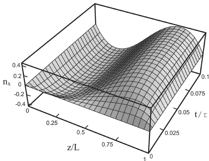
FIGURE 4 Three-dimensional time and space dependence of the director's x component after switching the laser radiation "on"; for homeotropic oriented cells with an approximation of strong anchoring.
